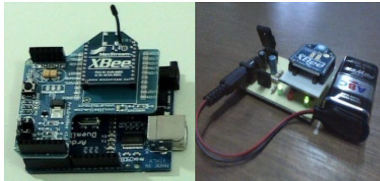
Gambar 5. Koordinator dan router/ end device
