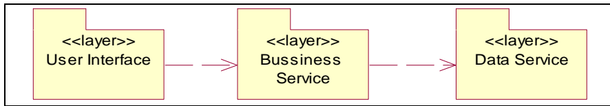
Gambar 4. System Design
