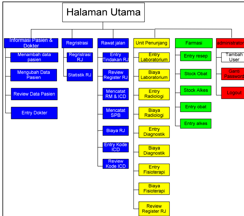
Gambar 12. Design Interface
